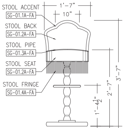
BAR STOOL - FRONT
