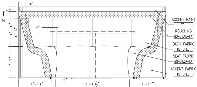
BANQUETTE (TYP.) - FRONT
