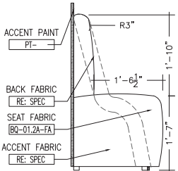
BANQUETTE (TYP.) - SECTION
