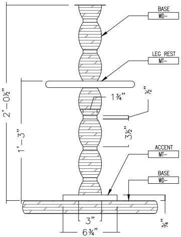
BAR STOOL - BASE DETAIL
