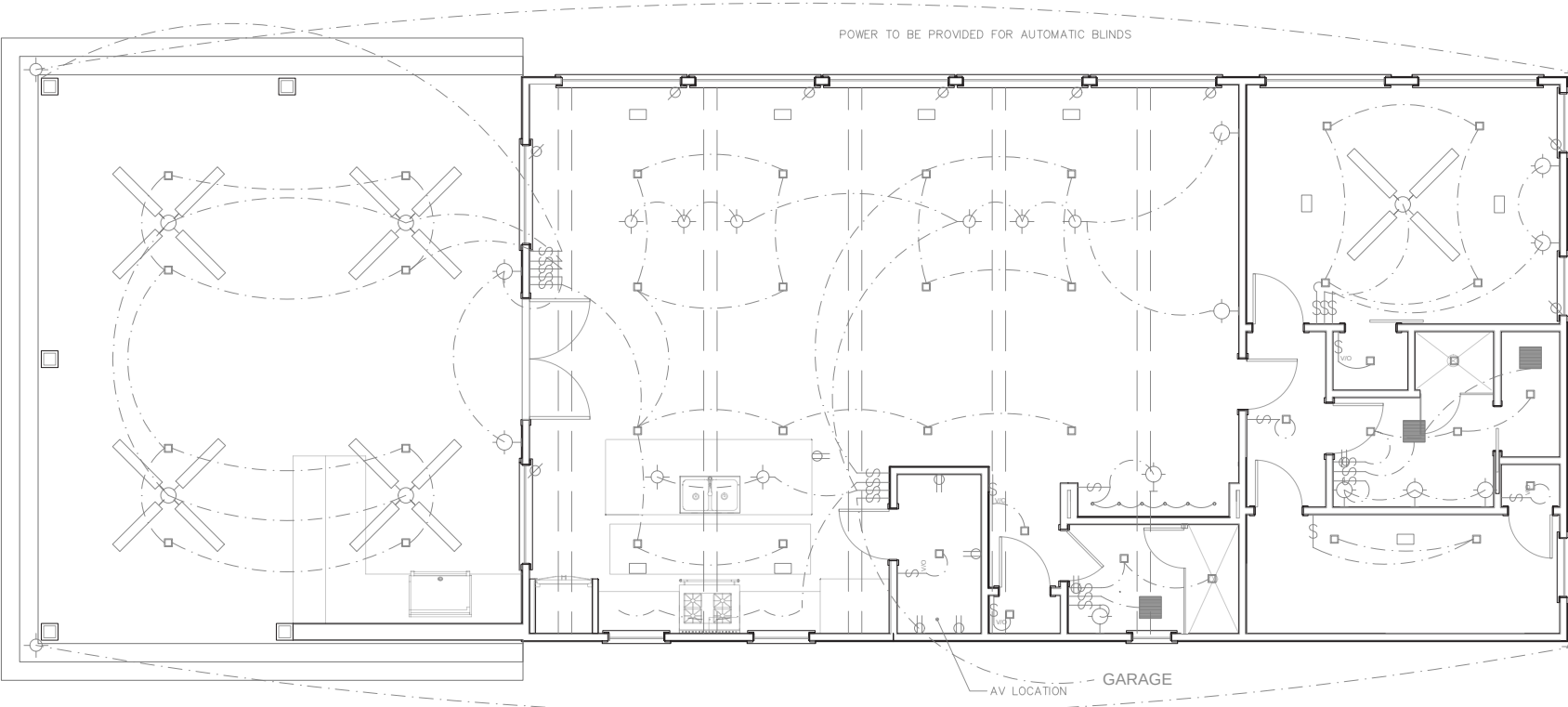
ELECTRICAL & LIGHTING PLAN
